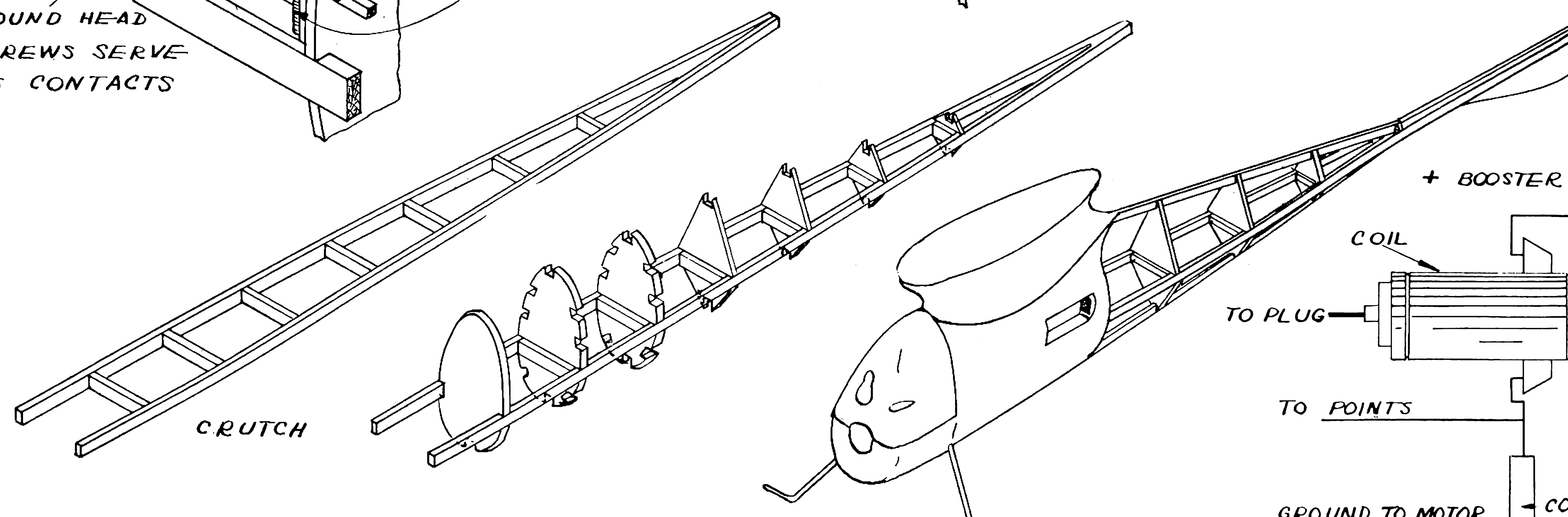
FUSELAGE CONSTRUCTION DETAILS.
